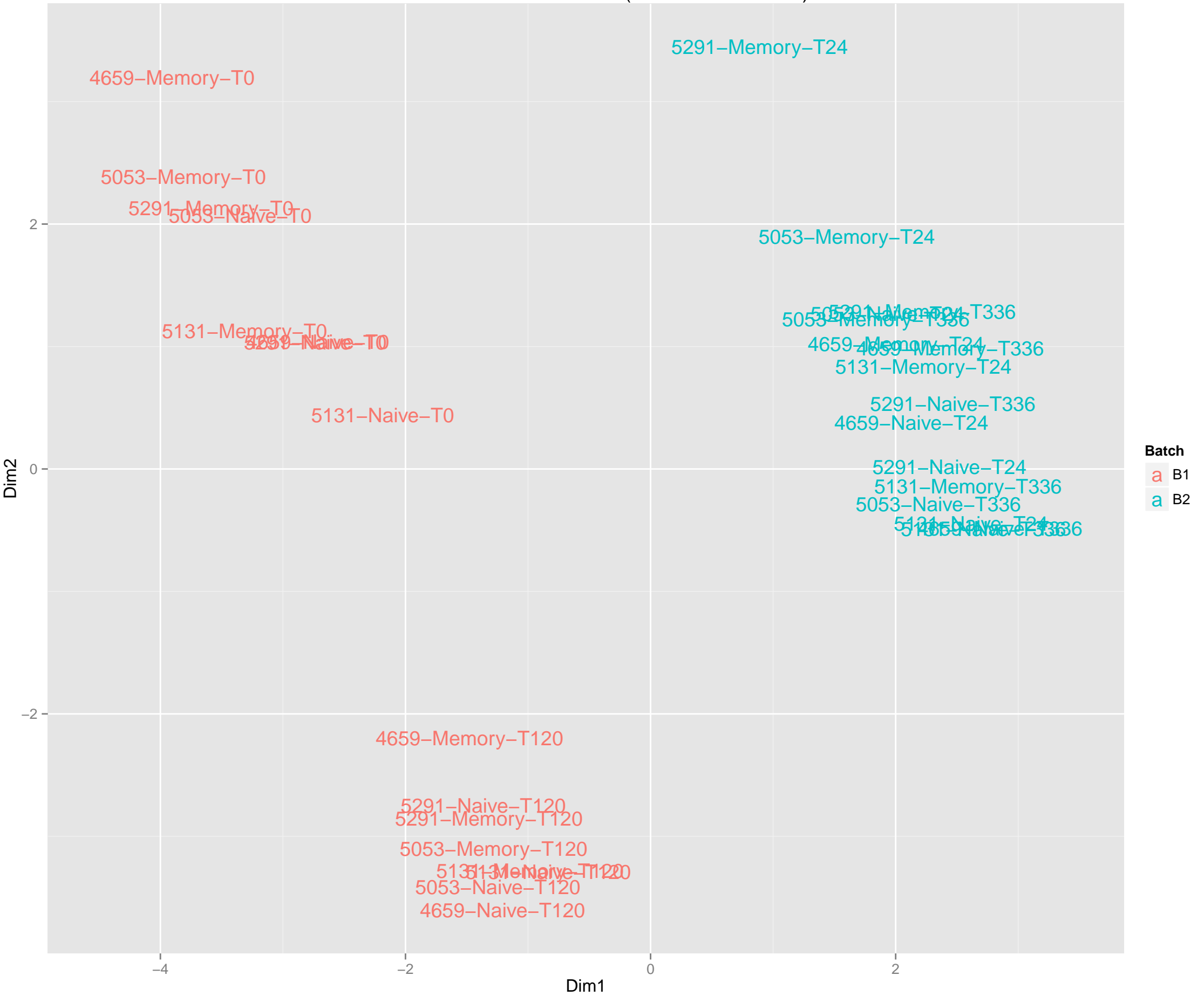
limma voom PC1 & 2 of data (no batch correction)
