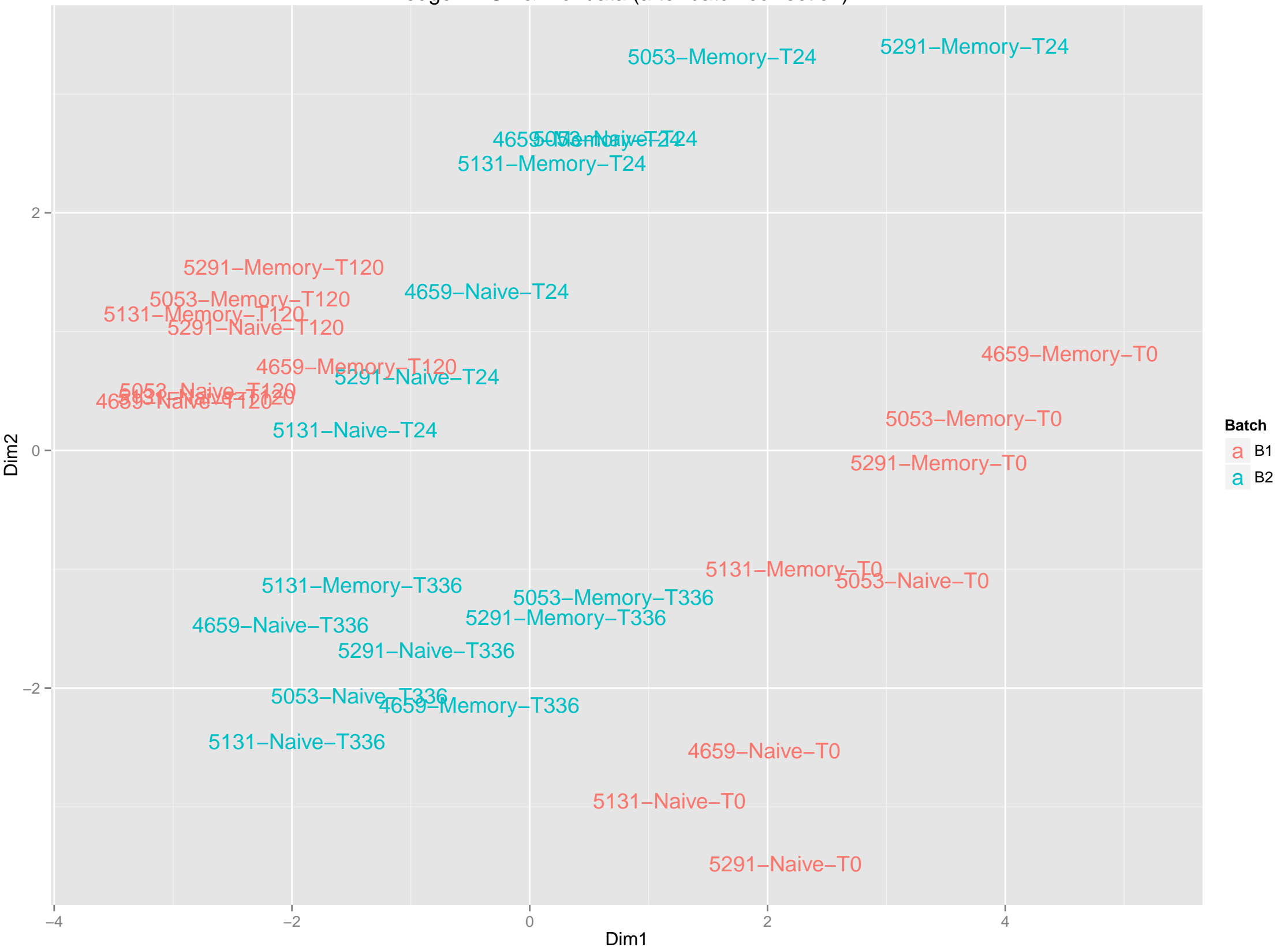
edgeR PC1 & 2 of data (after batch correction)
