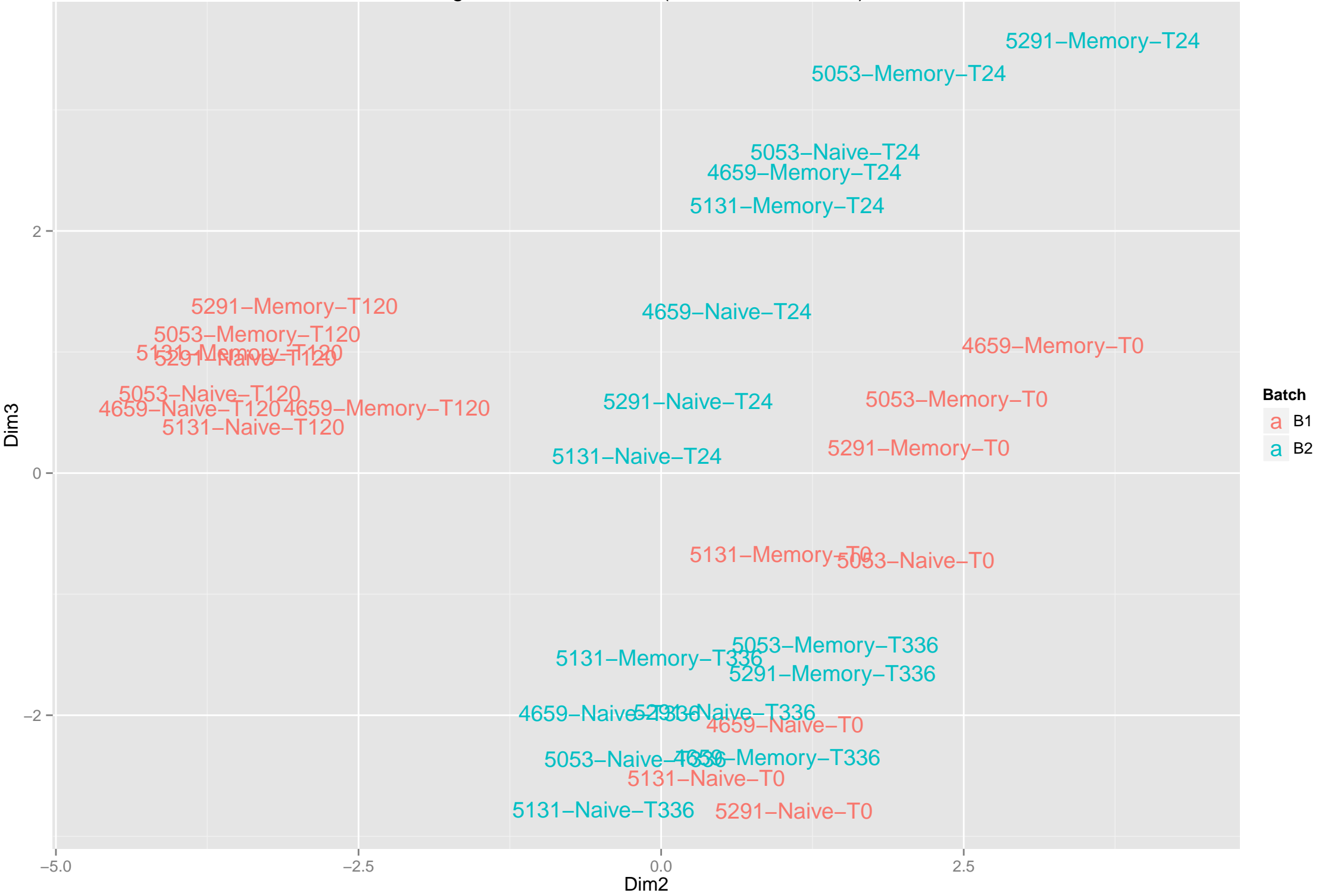
edgeR PC2 & 3 of data (no batch correction)
