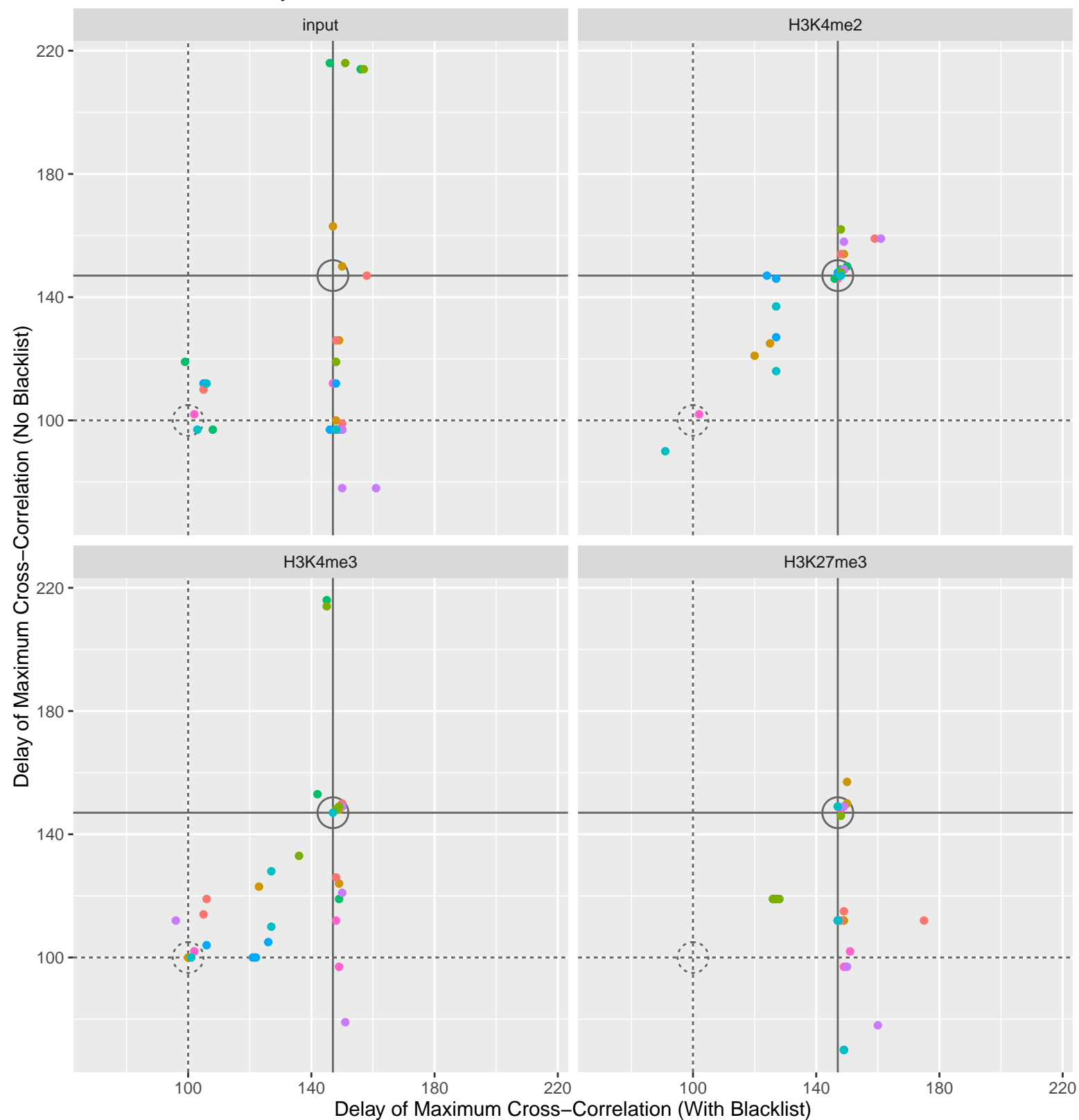
Delay of Maximum Cross-Correlation With and Without Blacklist
