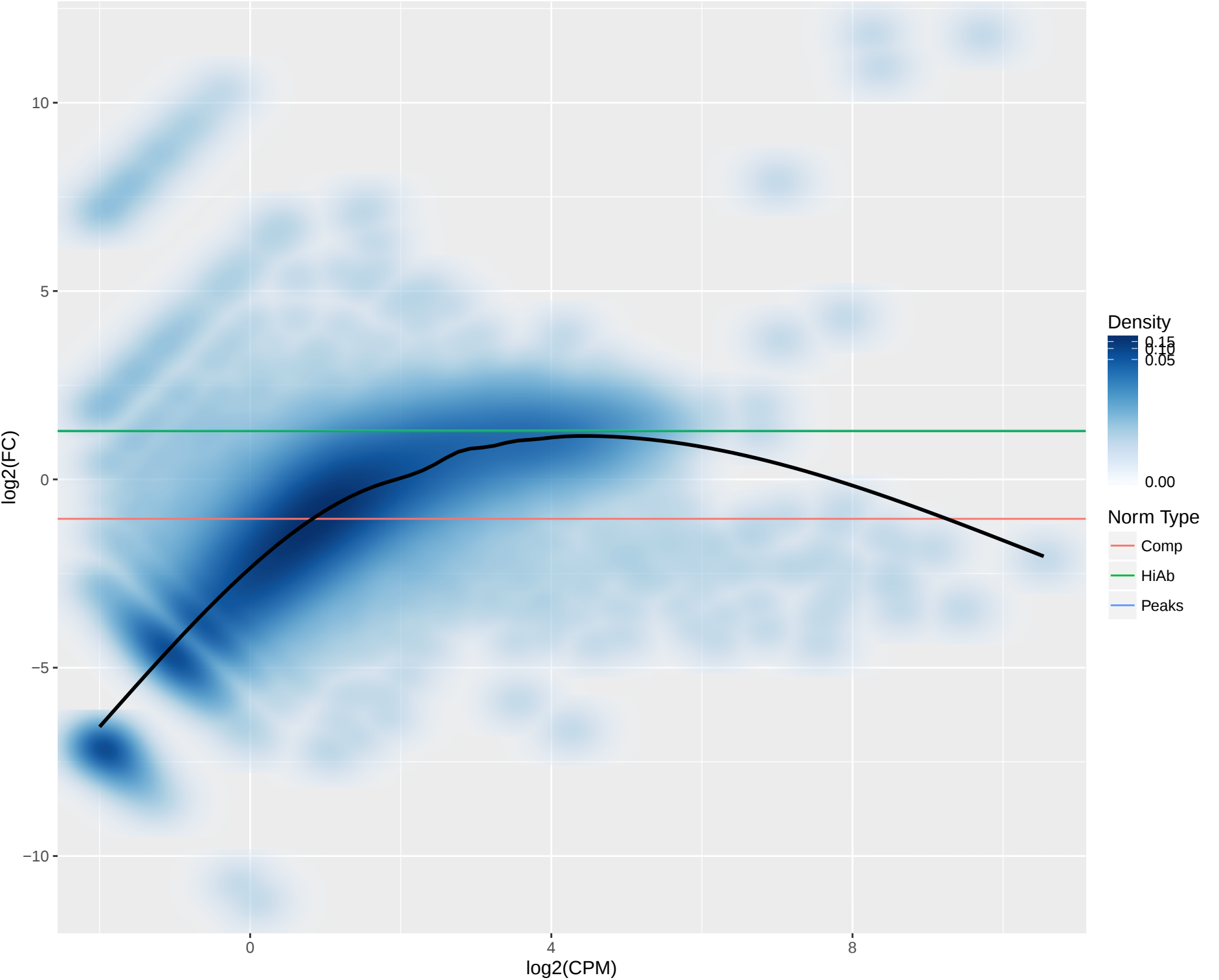
10KB Bin MA Plot for H3K4me3–Memory–D14–Donor5131 vs H3K4me3–Memory–D0–Donor5291
