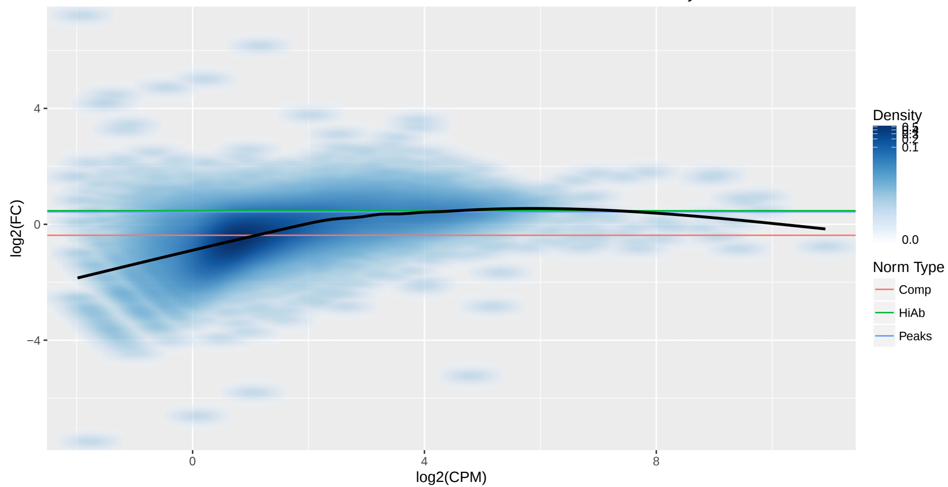
10KB Bin MA Plot for H3K4me3-Naive-D14-Donor5291 vs H3K4me3-Memory-D5-Donor4659
