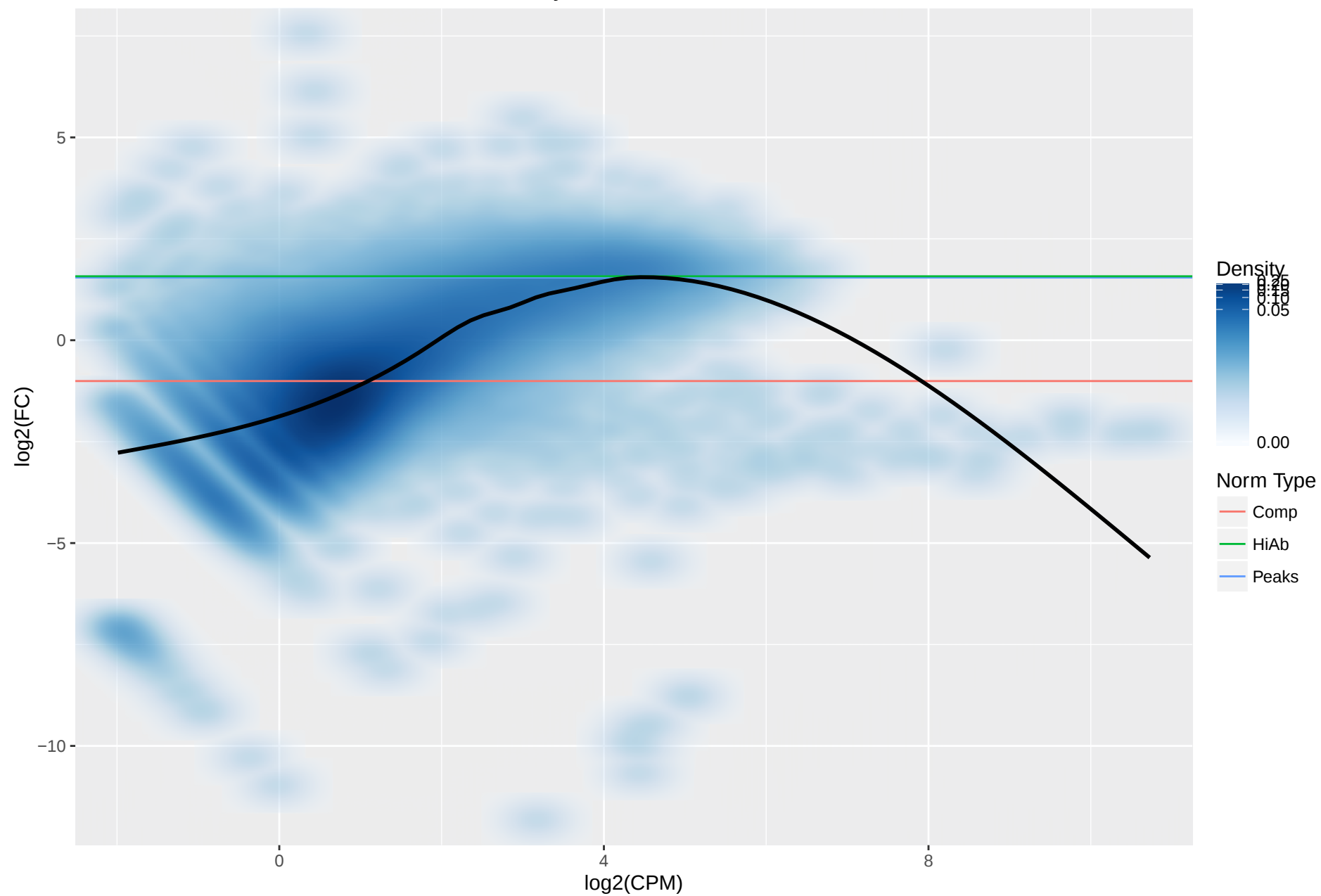
10KB Bin MA Plot for H3K4me3–Memory–D0–Donor5053 vs H3K4me3–Naive–D1–Donor5131
