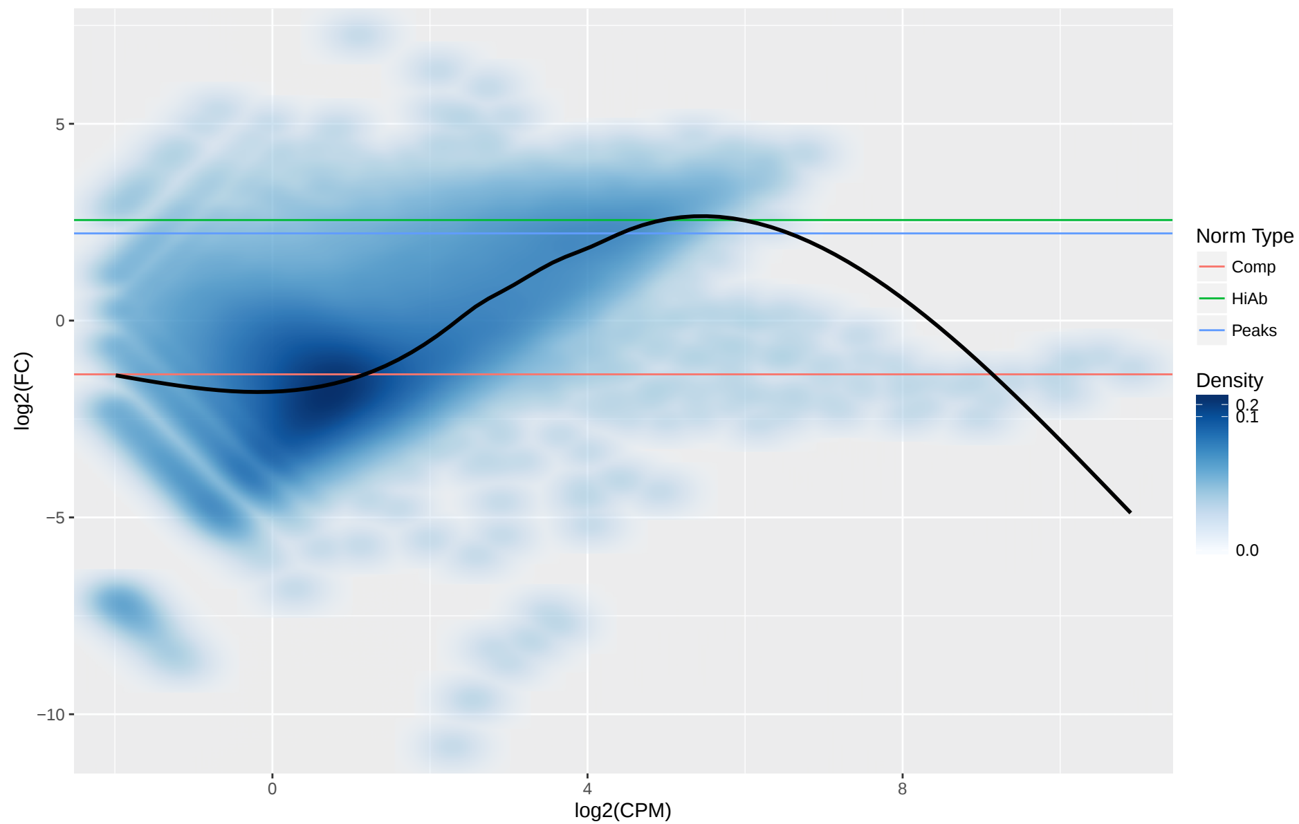
10KB Bin MA Plot for H3K4me3-Naive-D0-Donor4659 vs H3K4me3-Naive-D0-Donor5131
