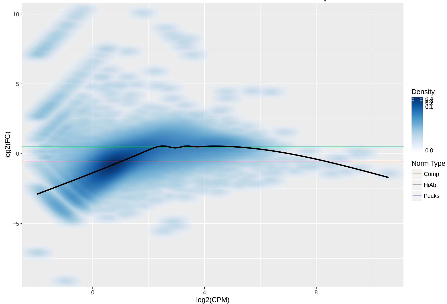
10KB Bin MA Plot for H3K4me3-Naive-D14-Donor5131 vs H3K4me3-Memory-D1-Donor5053
