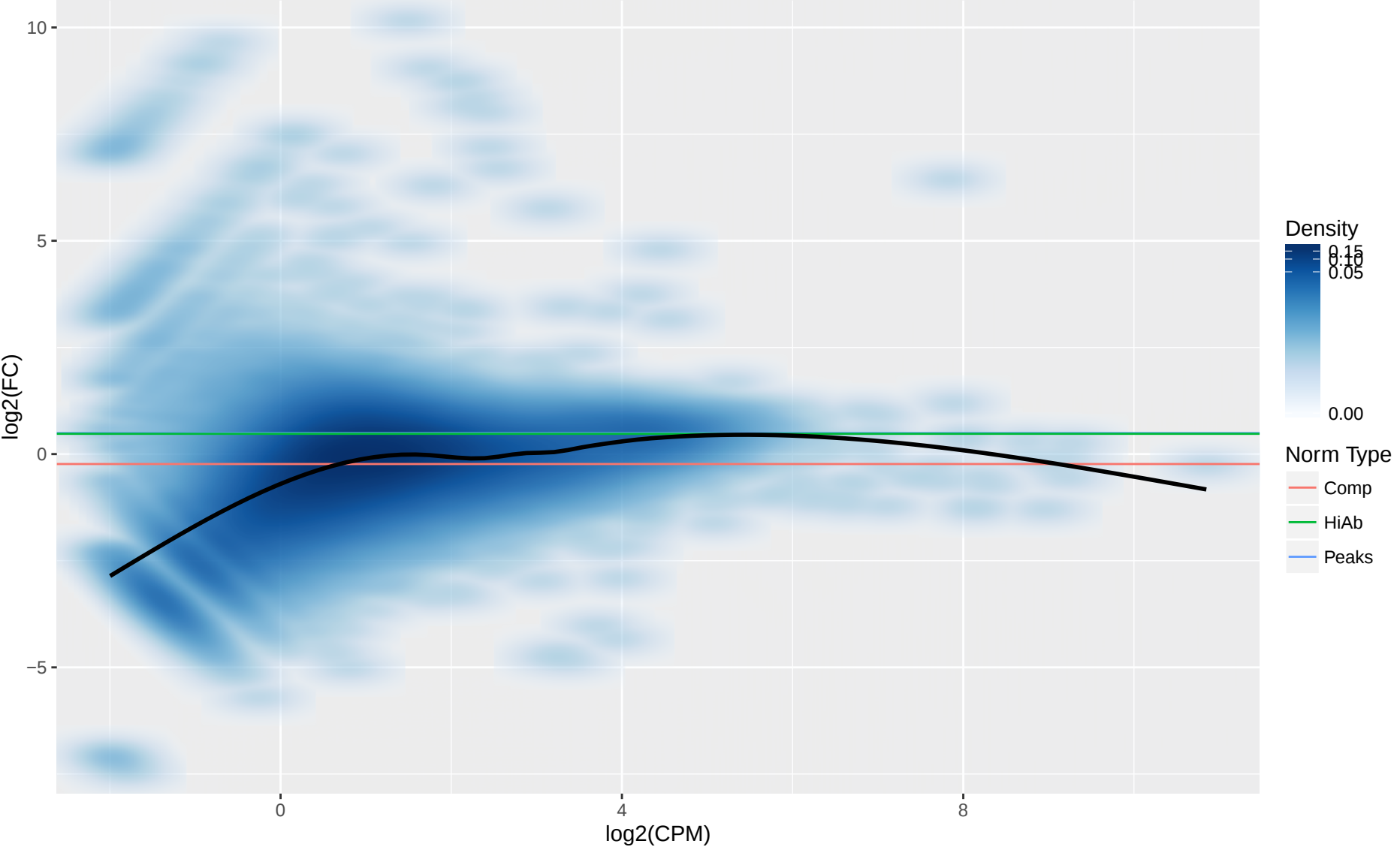
10KB Bin MA Plot for H3K4me3–Memory–D5–Donor5131 vs H3K4me3–Memory–D5–Donor5291
