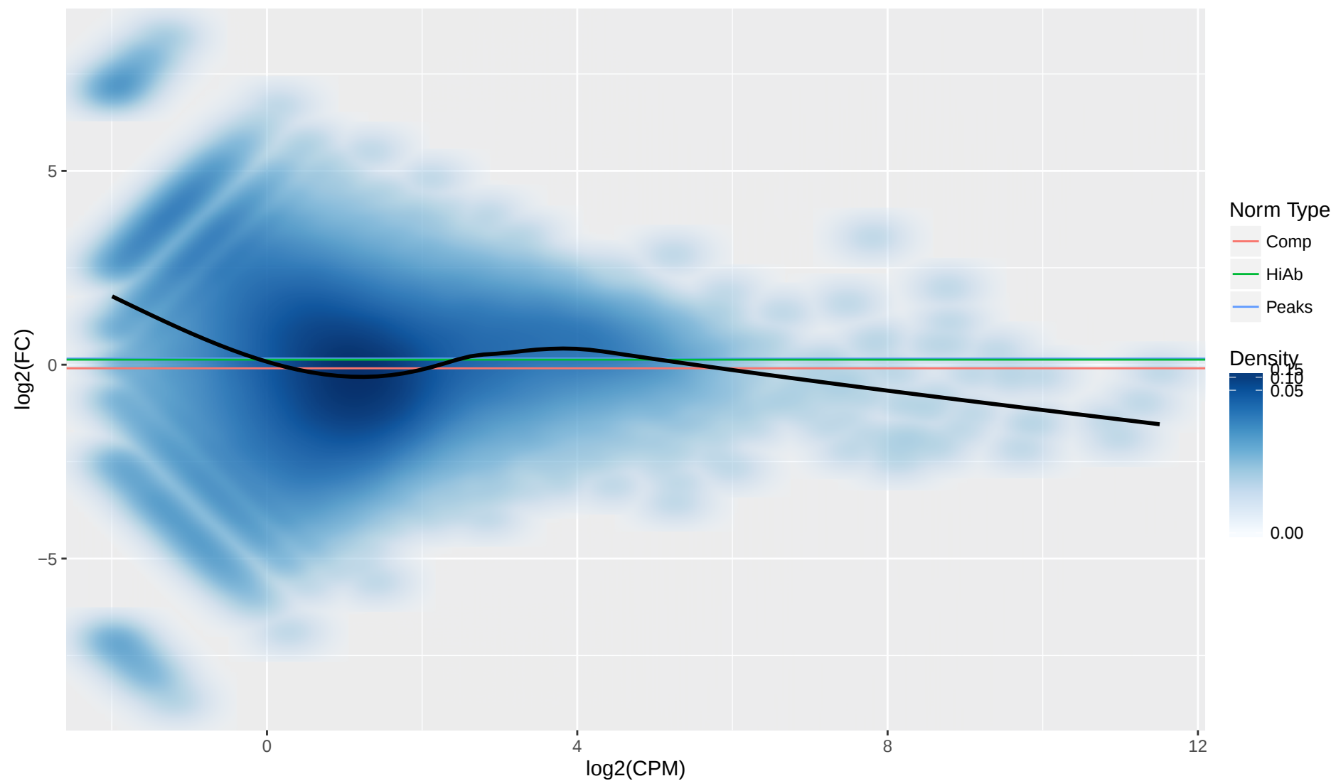
10KB Bin MA Plot for H3K4me3-Naive-D0-Donor5053 vs H3K4me3-Naive-D0-Donor5291
