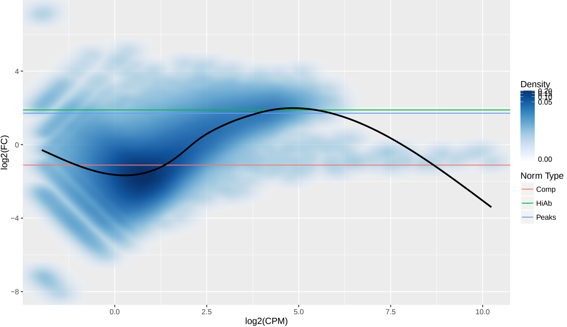
10KB Bin MA Plot for H3K4me3–Naive–D5–Donor5053 vs H3K4me3–Naive–D1–Donor5053
