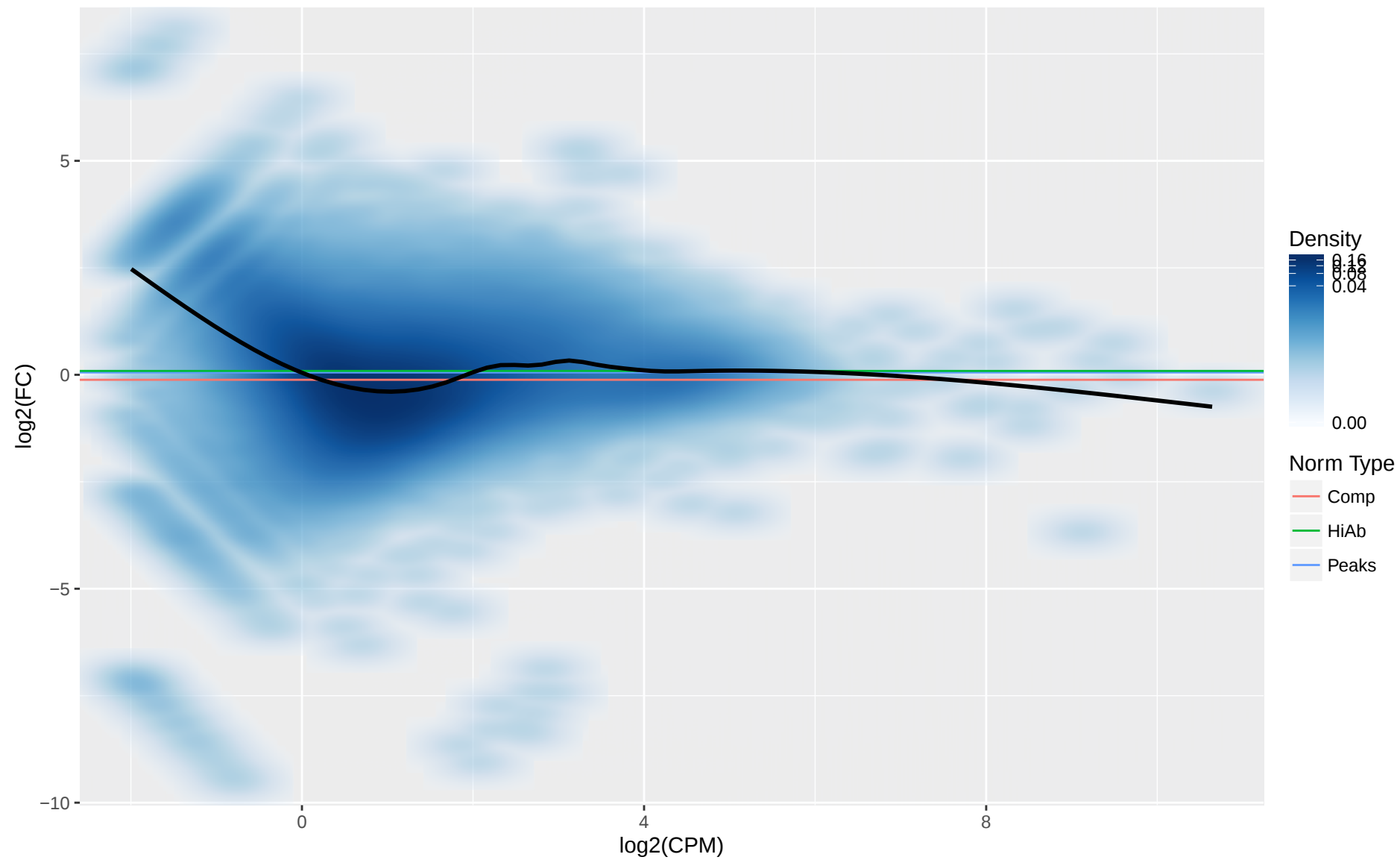
10KB Bin MA Plot for H3K4me3–Naive–D5–Donor5291 vs H3K4me3–Memory–D1–Donor5131
