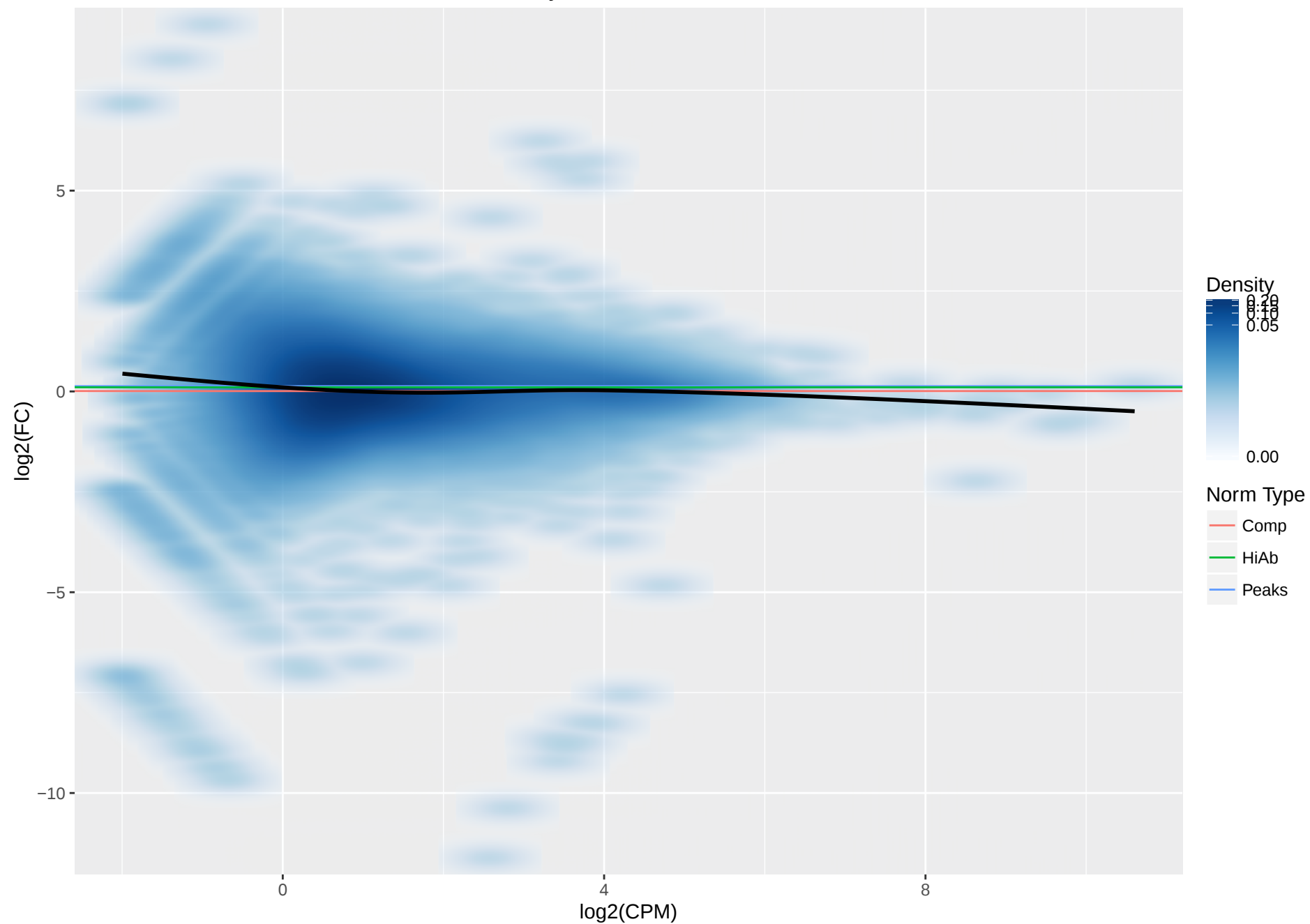
10KB Bin MA Plot for H3K4me3–Memory–D5–Donor5053 vs H3K4me3–Naive–D5–Donor5131
