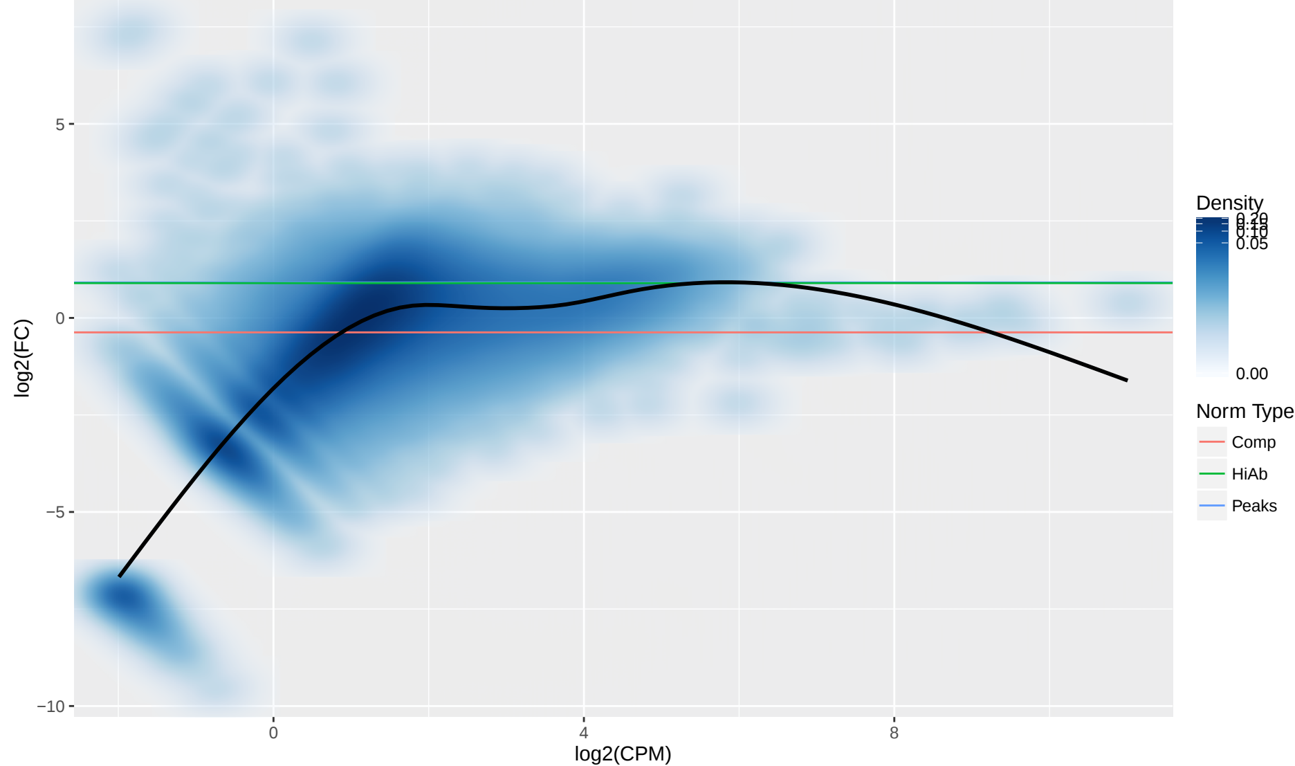
10KB Bin MA Plot for H3K4me3–Memory–D14–Donor5053 vs H3K4me3–Memory–D1–Donor5291
