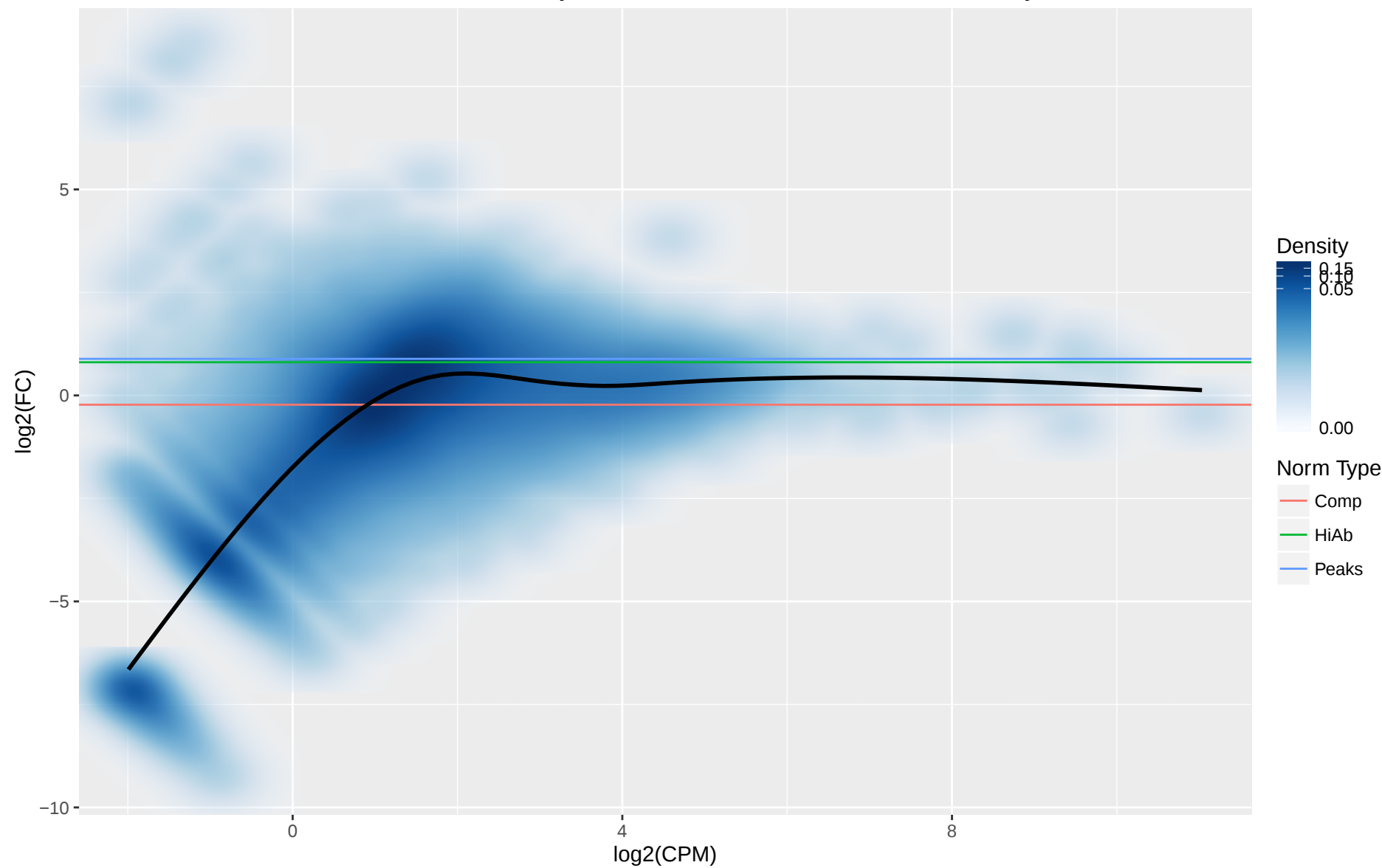
10KB Bin MA Plot for H3K4me3–Memory–D14–Donor5291 vs H3K4me3–Memory–D1–Donor4659
