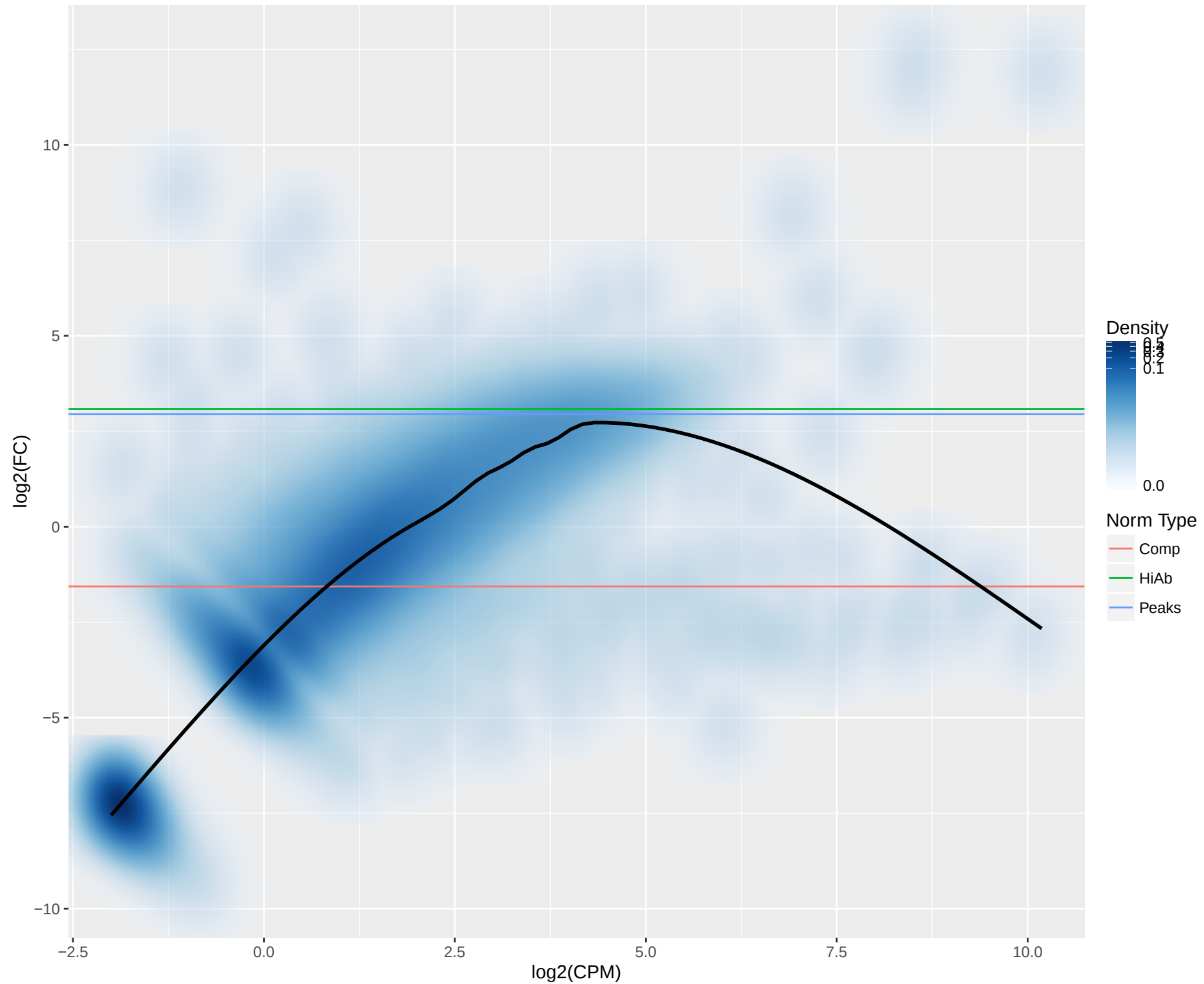
10KB Bin MA Plot for H3K4me3–Naive–D14–Donor5053 vs H3K4me3–Memory–D0–Donor4659
