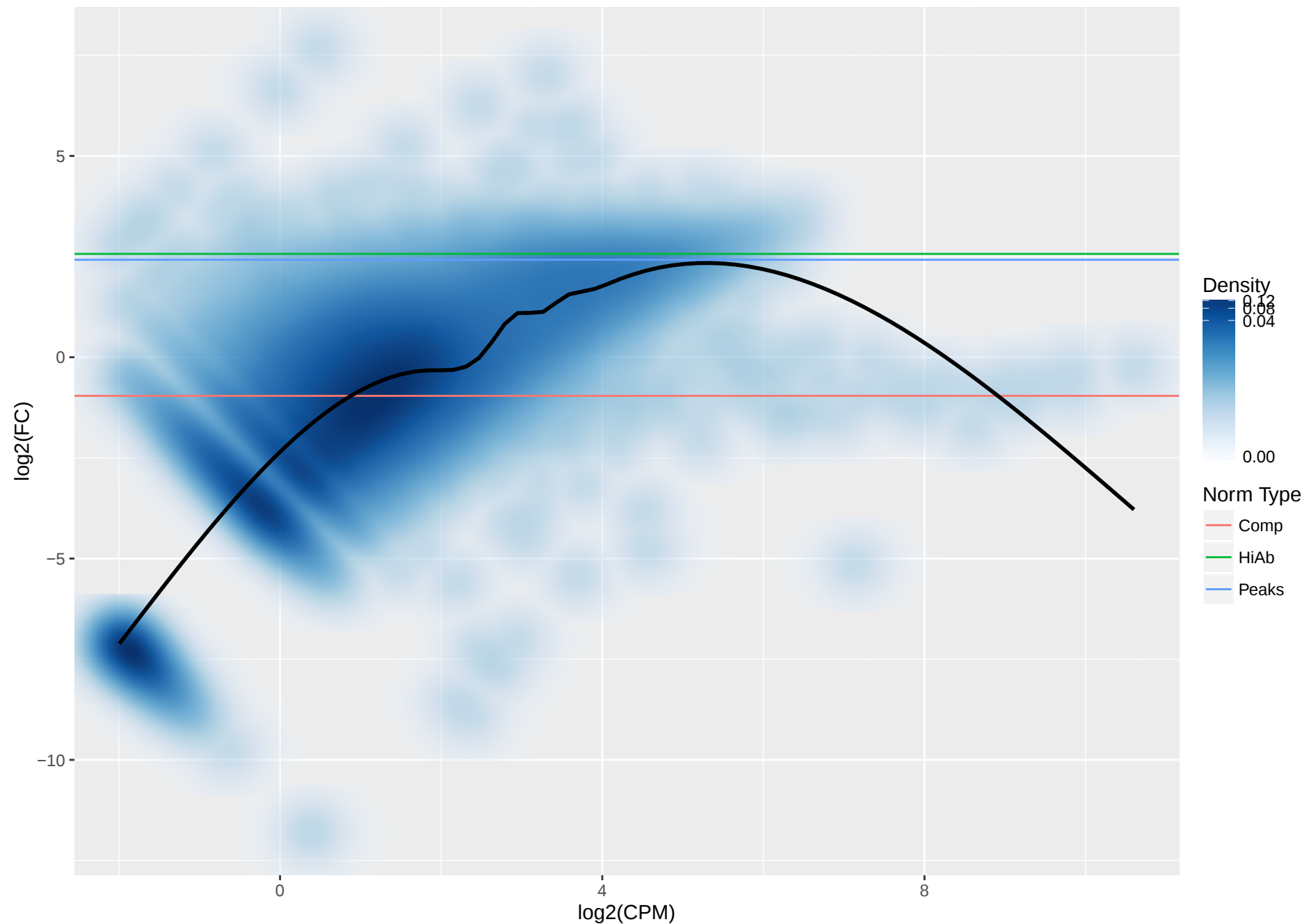
10KB Bin MA Plot for H3K4me3–Memory–D14–Donor4659 vs H3K4me3–Memory–D0–Donor5131
