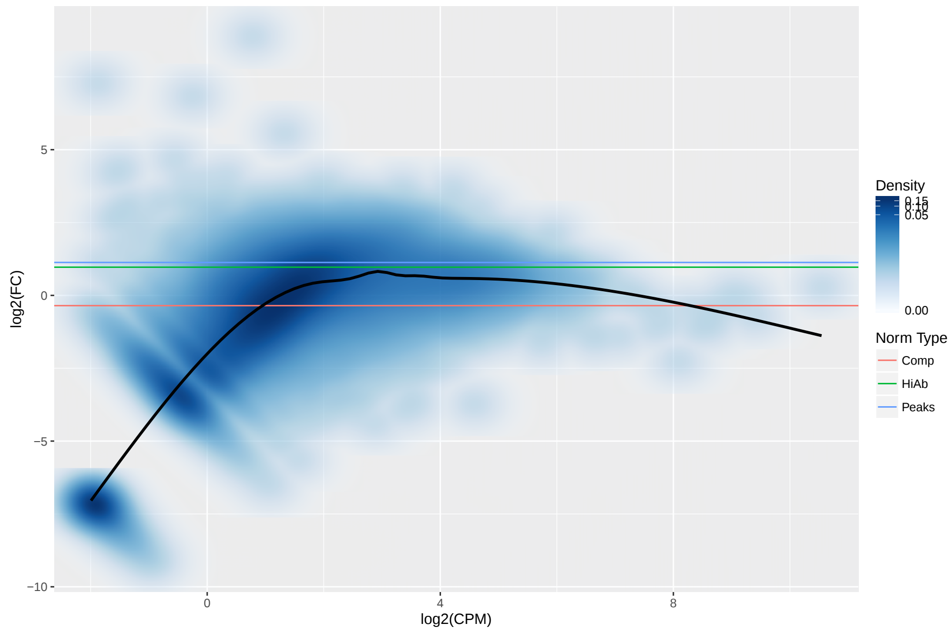
10KB Bin MA Plot for H3K4me3-Naive-D14-Donor4659 vs H3K4me3-Naive-D1-Donor5291
