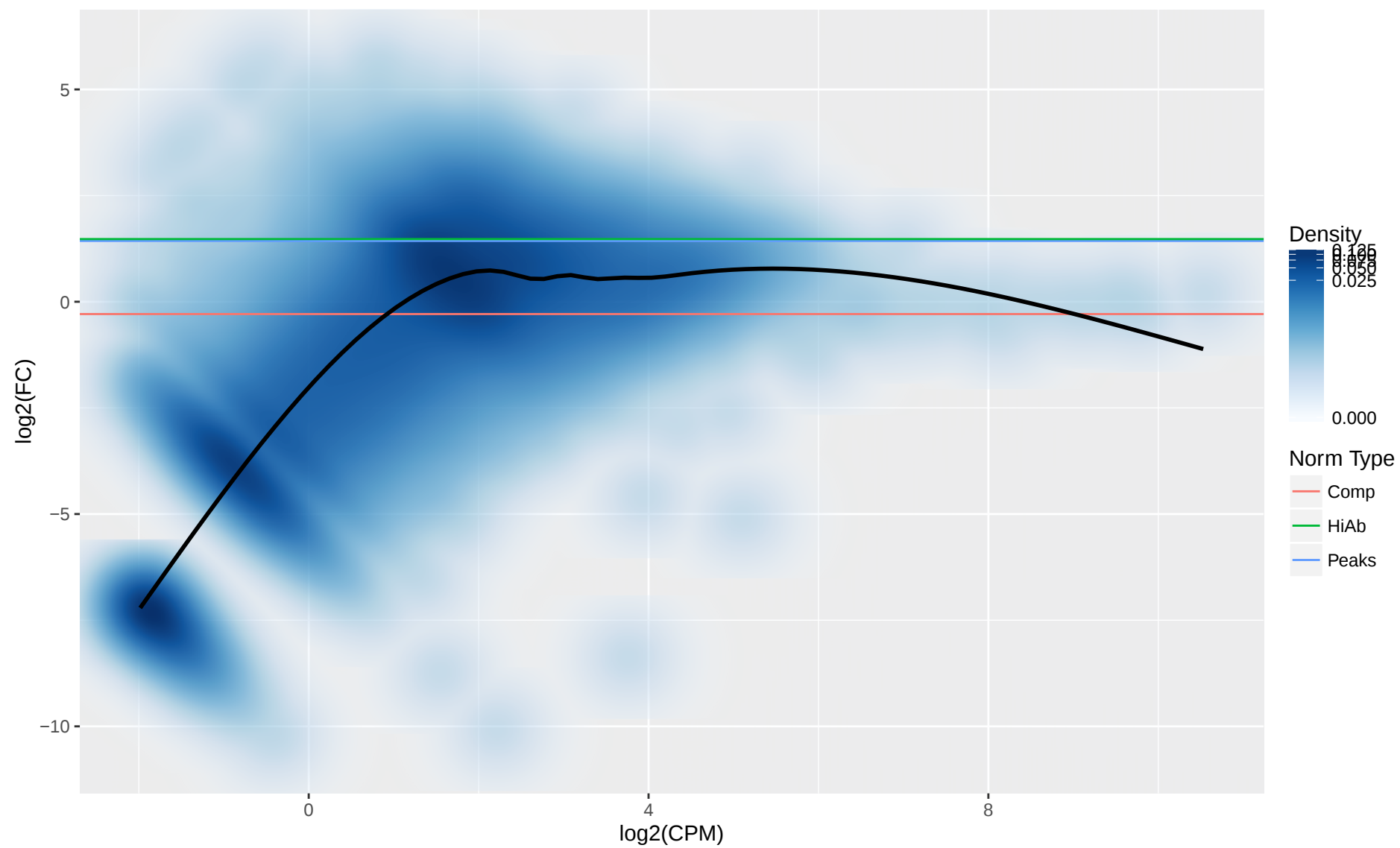
10KB Bin MA Plot for H3K4me3-Naive-D5-Donor4659 vs H3K4me3-Naive-D1-Donor4659
