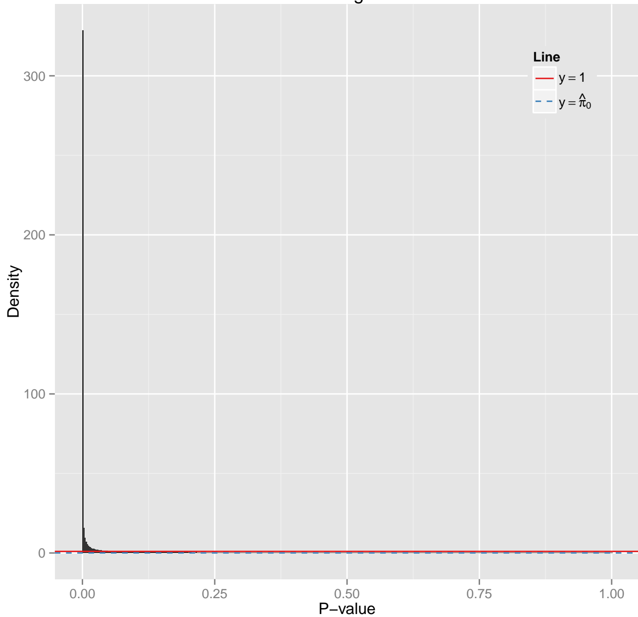
P-value histogram for SV
