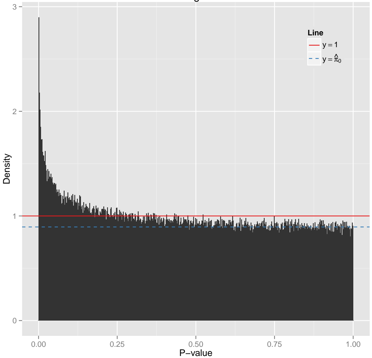
P-value histogram for MvsF
