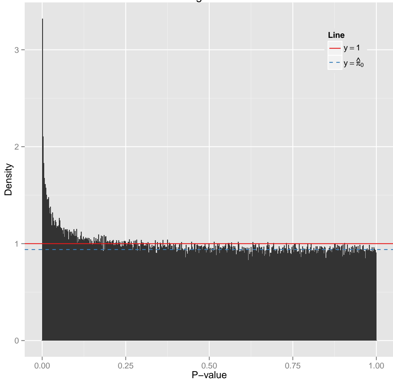
P-value histogram for CANvsTX
