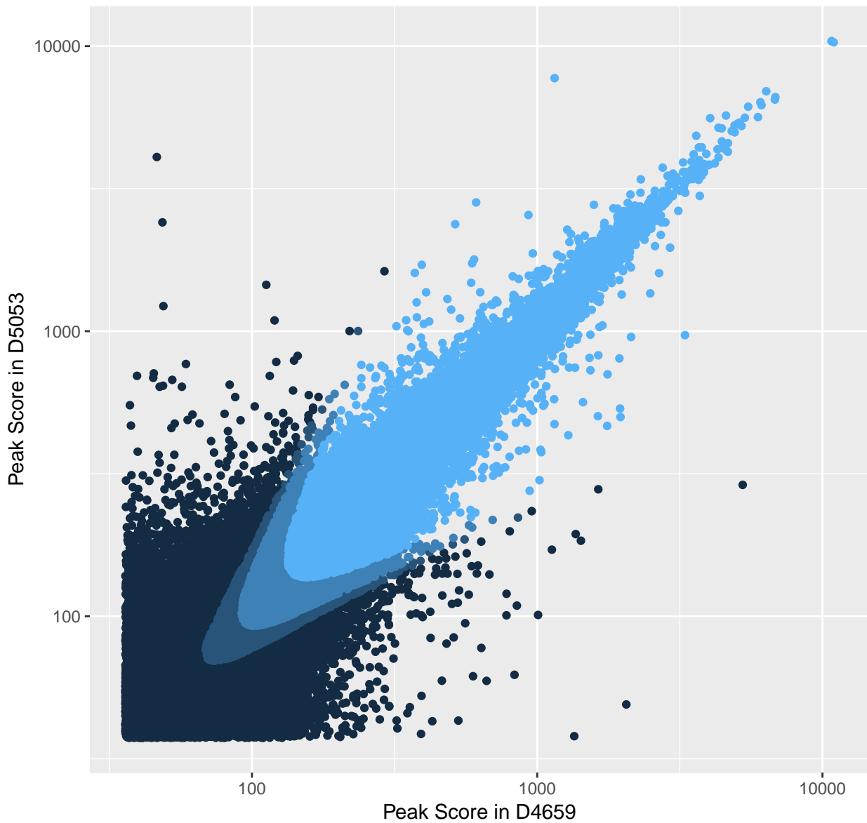
Score consistency plot for H3K27me3-ALL, D4659 vs D5053
