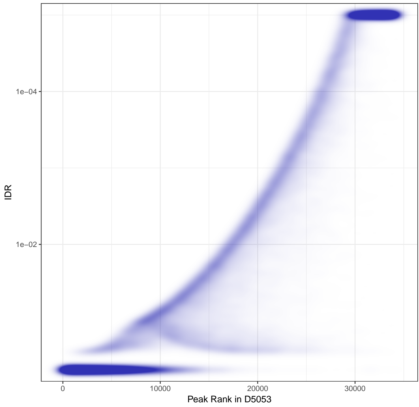
IDR vs Peak Rank for H3K27me3-ALL D5053
