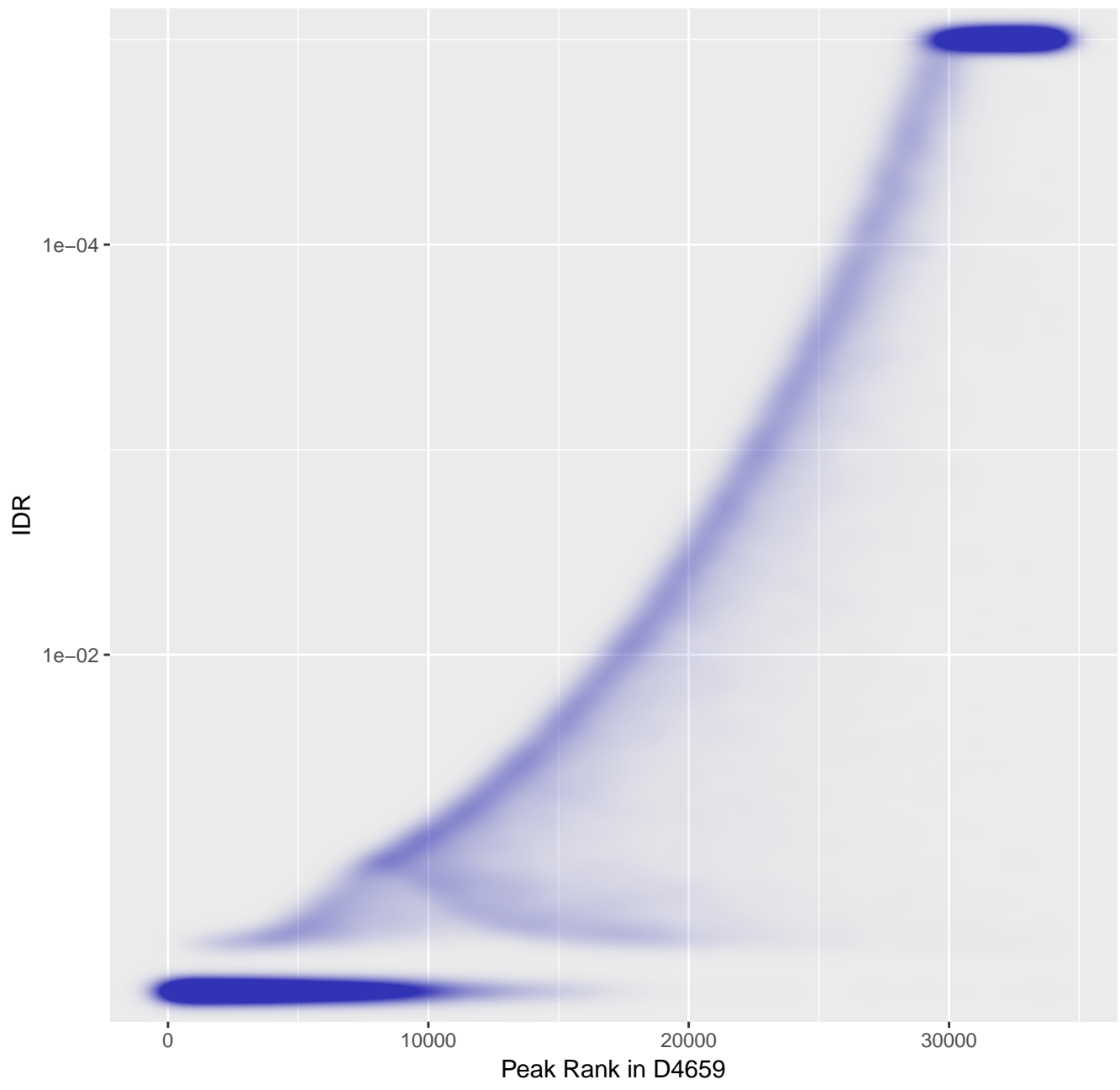
IDR vs Peak Rank for H3K27me3-ALL D4659
