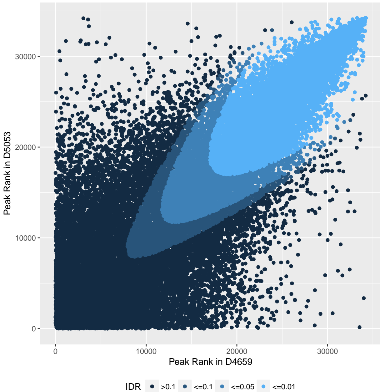
Rank consistency plot for H3K27me3-ALL, D4659 vs D5053
